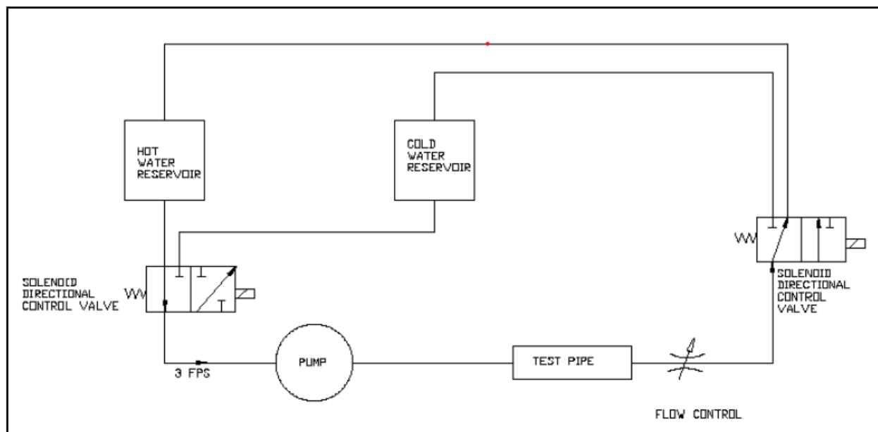
Figure 2: Schematic of time response test apparatus
